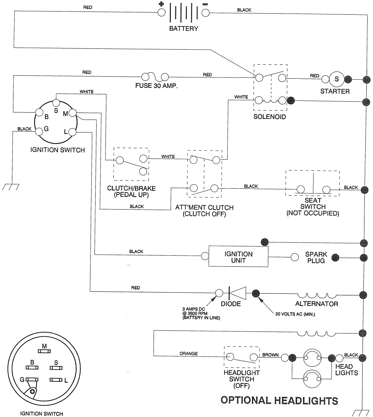
IGNITION SWITCH
