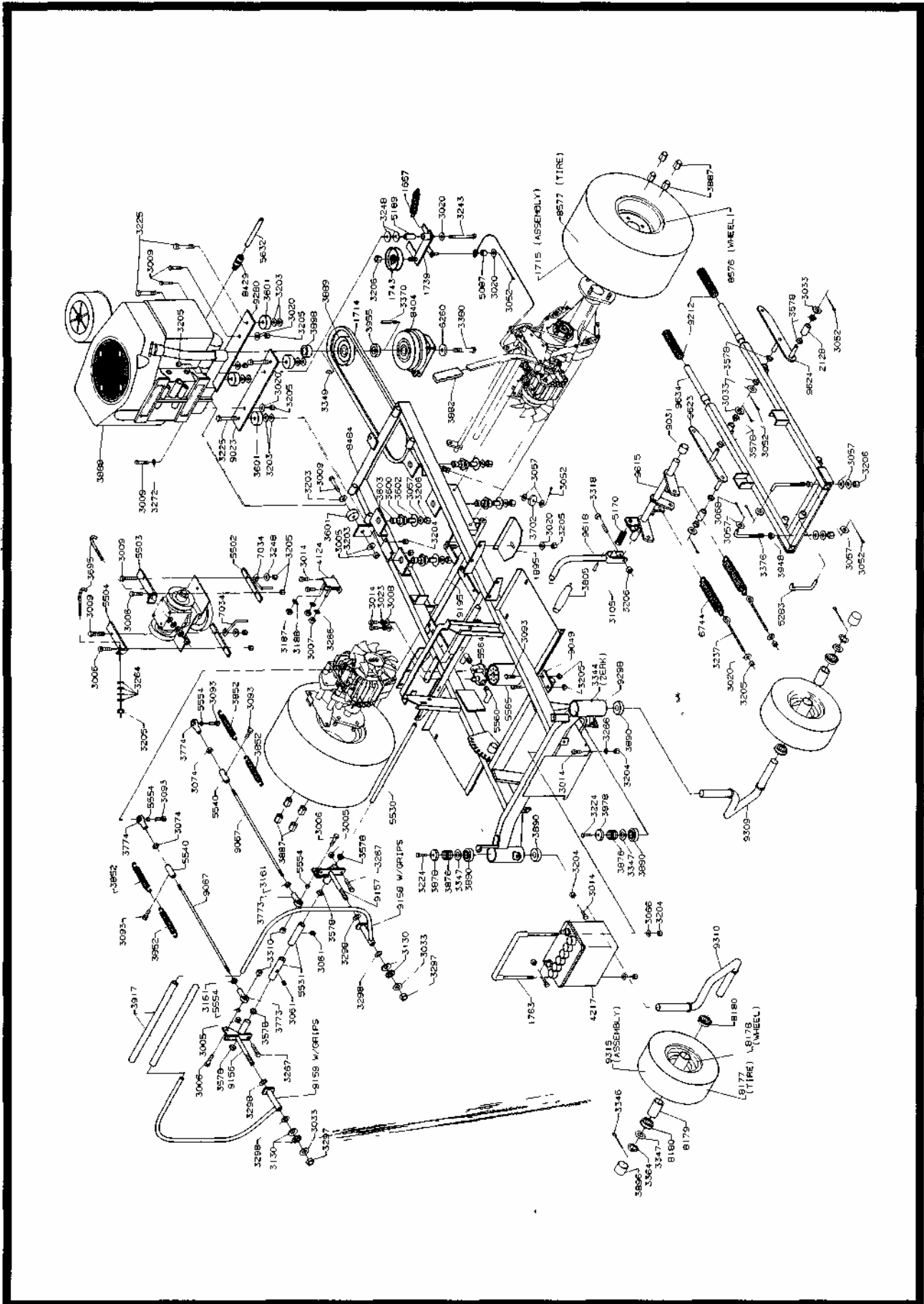
560 Chassis Assembly
