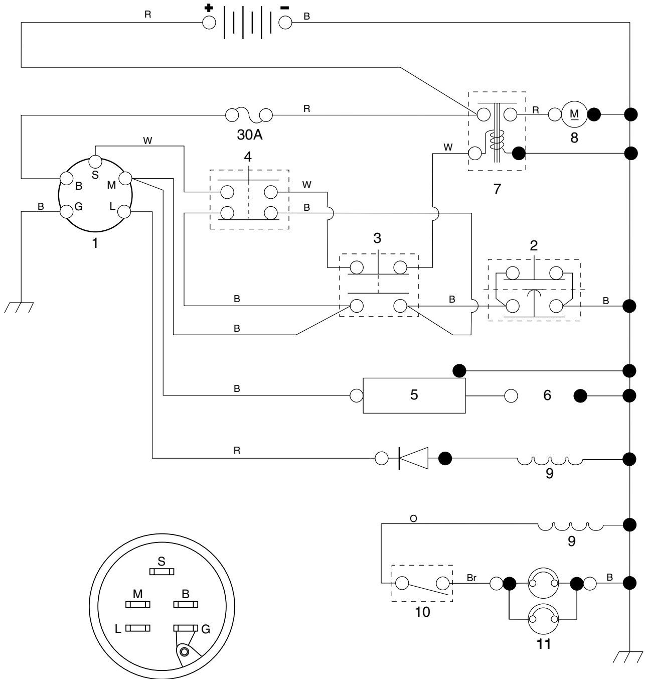
Ignition switch
