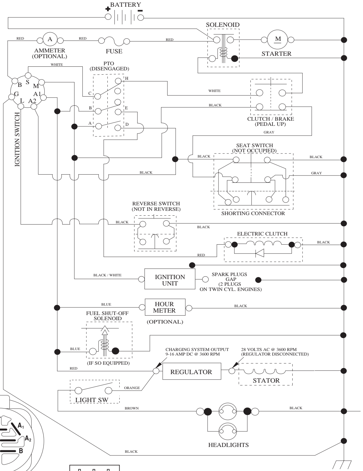
IGNITION SWITCH
