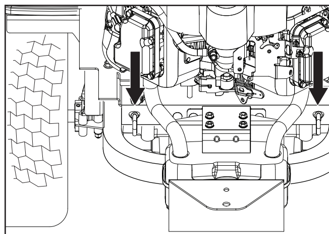
Bypass linkages
