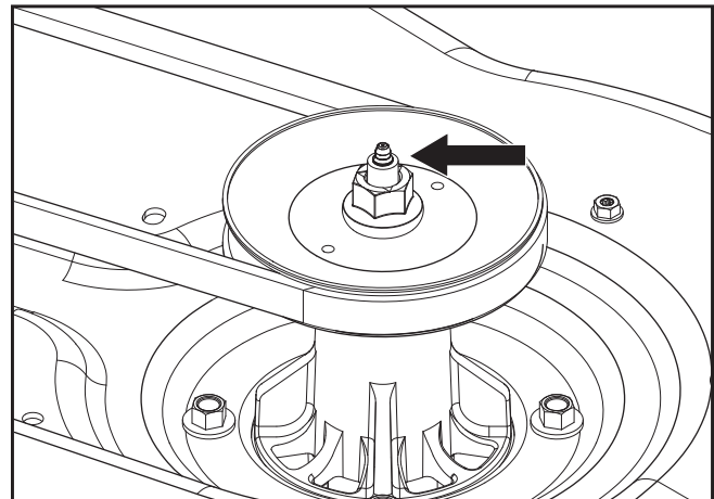
Deck spindle
