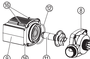
FSP 8500 Economic
