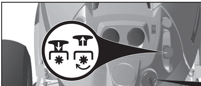
☒ ) ATTACHMENT CLUTCH SWITCH "DISENGAGED" ☑ ) ATTACHMENT CLUTCH SWITCH "ENGAGED"
