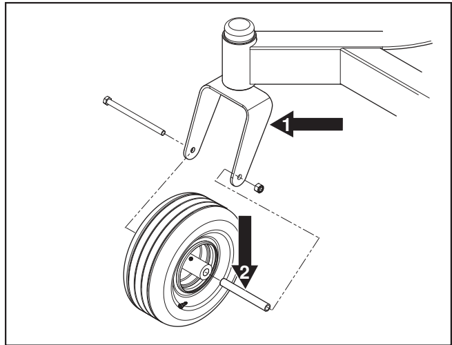
Caster wheels
