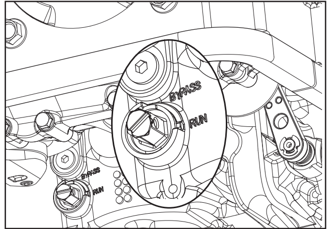
Right side, ZT-5400 bypass valve
