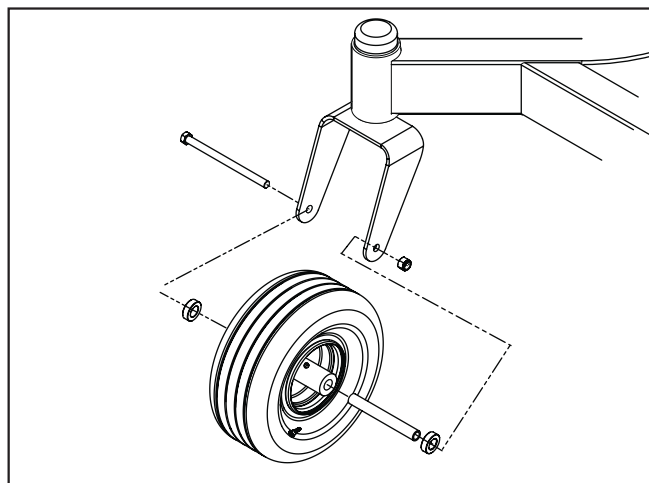
Caster wheels
