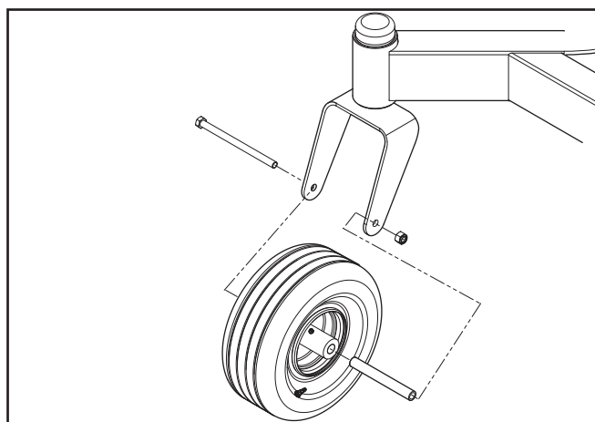
Caster wheel
