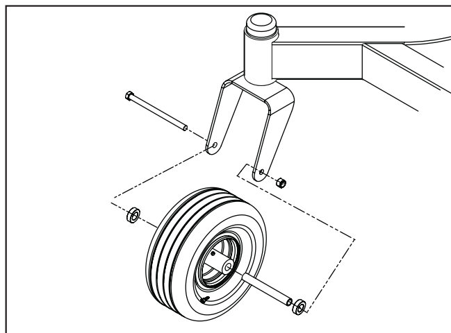
Caster wheels
