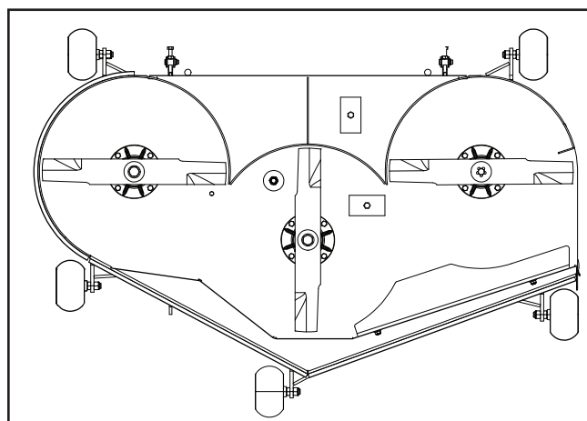
Set blades to begin alignment
