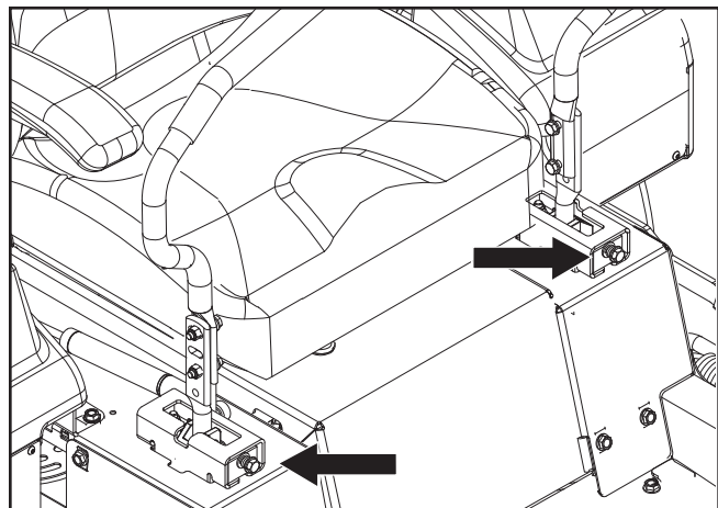
Tracking bolts
