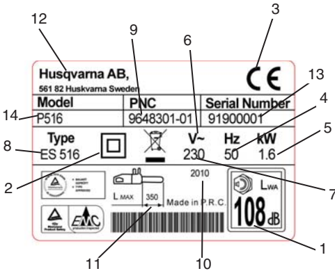
Example of identification label
